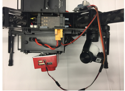
XT30 connector plugged into distribution board
