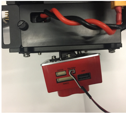
RedEdge-M connector of BEC plugged into RedEdge-M power port
