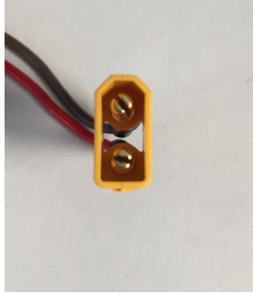
XT30 connector, note gender keying
