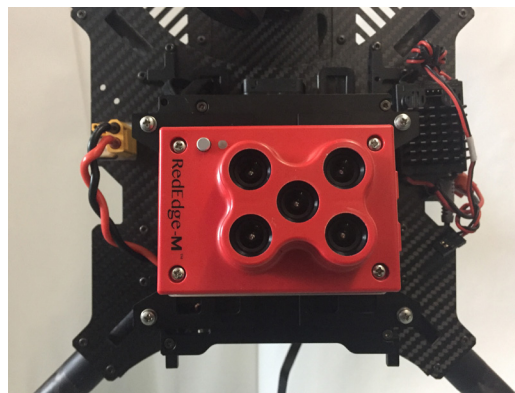
RedEdge-M and mount screwed into Matrice 100 battery cover
