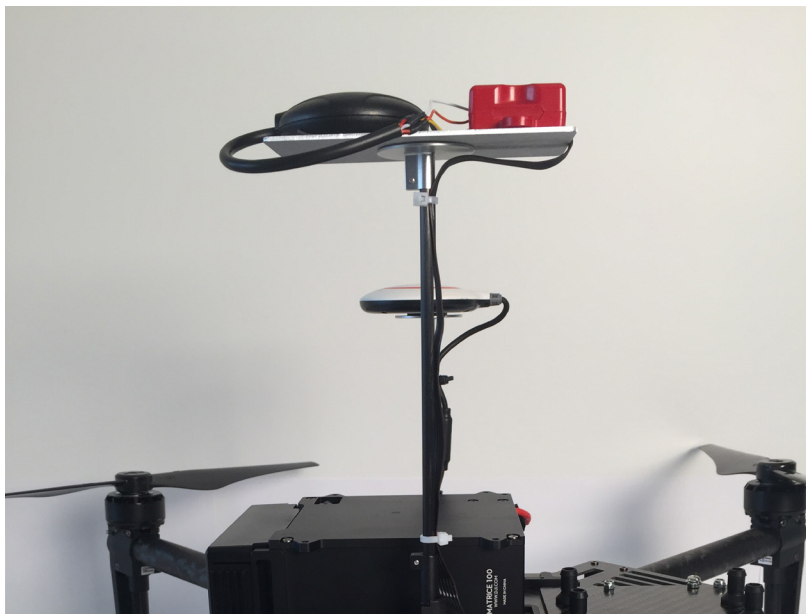
DLS and GPS attached to mounting plate.
