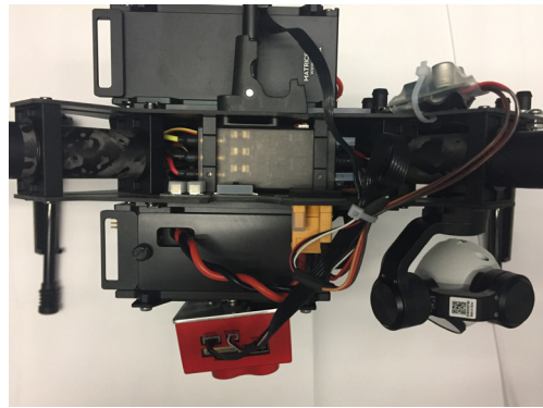
BEC attached to airframe using included VHB tape and zip ties.
